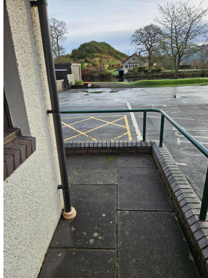
Protruding Downpipe
